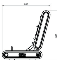
side view open position
